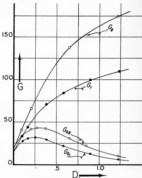
FIG. 9. G - D diagram: G_1 and G_2 are the graininess-density functions of two different emulsions from which G_{s1} and G_{s2} have been derived by transformation.
